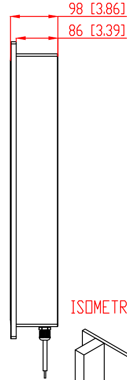
SIDE VIEW ON SPEAKER
