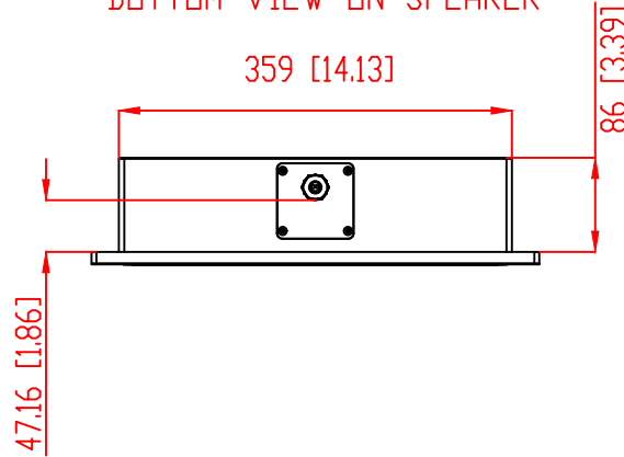
BOTTOM VIEW ON SPEAKER
